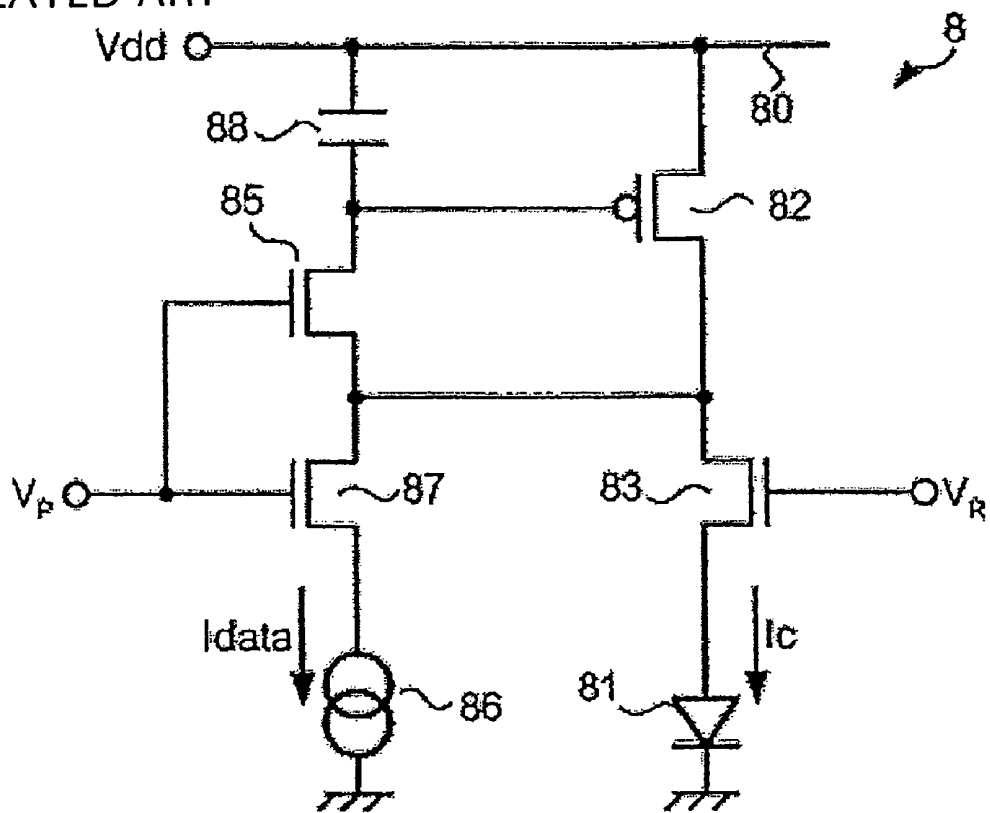
FIG.16 RELATED ART
