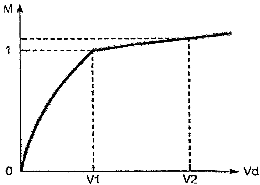
FIG.17 RELATED ART
